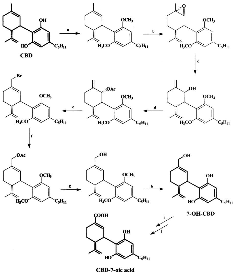
Fig. 9. Synthesis of 7-OH-CBD and CBD-7-oic acid. (a) \text{CH}_3\text{I} , \text{K}_2\text{CO}_3 in DMF; (b) 3-chloro-perbenzoic acid in \text{CH}_2\text{CK}_2 ; (c) methylmagnesium bromide, N-cyclohexylisopropylamine in toluene; (d) acetic anhydride in pyridine; (e) t-butyl-dimethyl-silyl bromide in \text{CH}_2\text{Cl}_2 ; (f) tetrabutylammonium acetate in acetone; (g) \text{NaOH} aq; (h) \text{CH}_3\text{MgI} at 200^\circ\text{C} ; (i) blocking of phenolic groups; (j) oxidation of allylic alcohol to acid.
